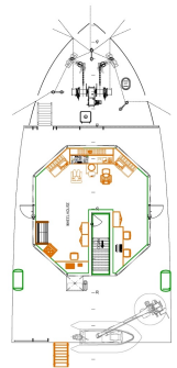
BRIDGE DECK
