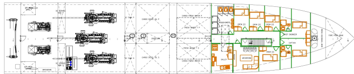
LOWER DECK
